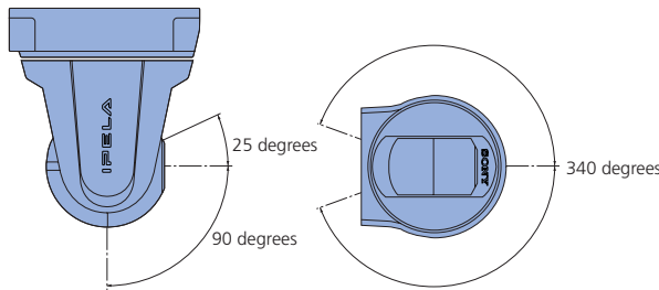
Fig. 1 Pan/Tilt Range
